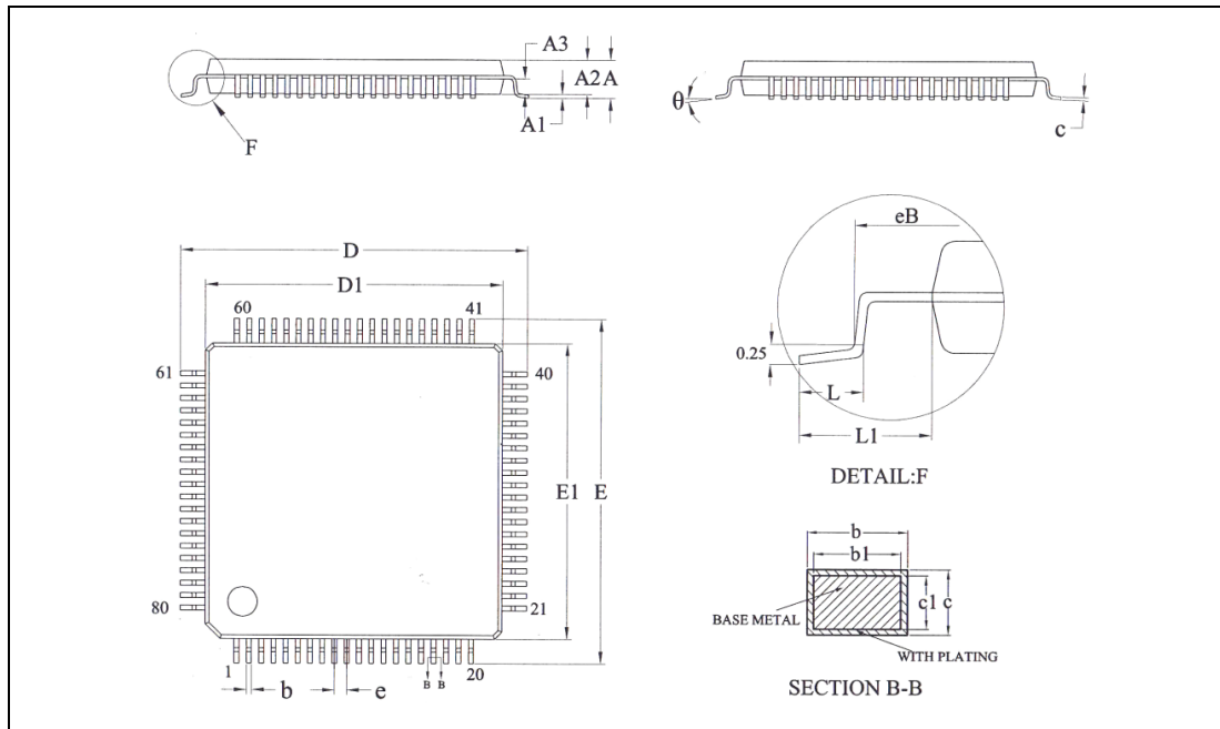
Figure 18. LQFP80 - 80 pin, 12 x 12 mm low-profile quad flat package outline
