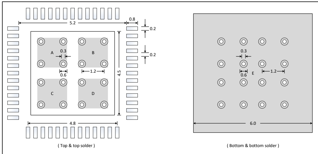
Figure 27. QFN52 - 52 pin, 6 x 6 mm quad flat no-lead package recommended footprint
