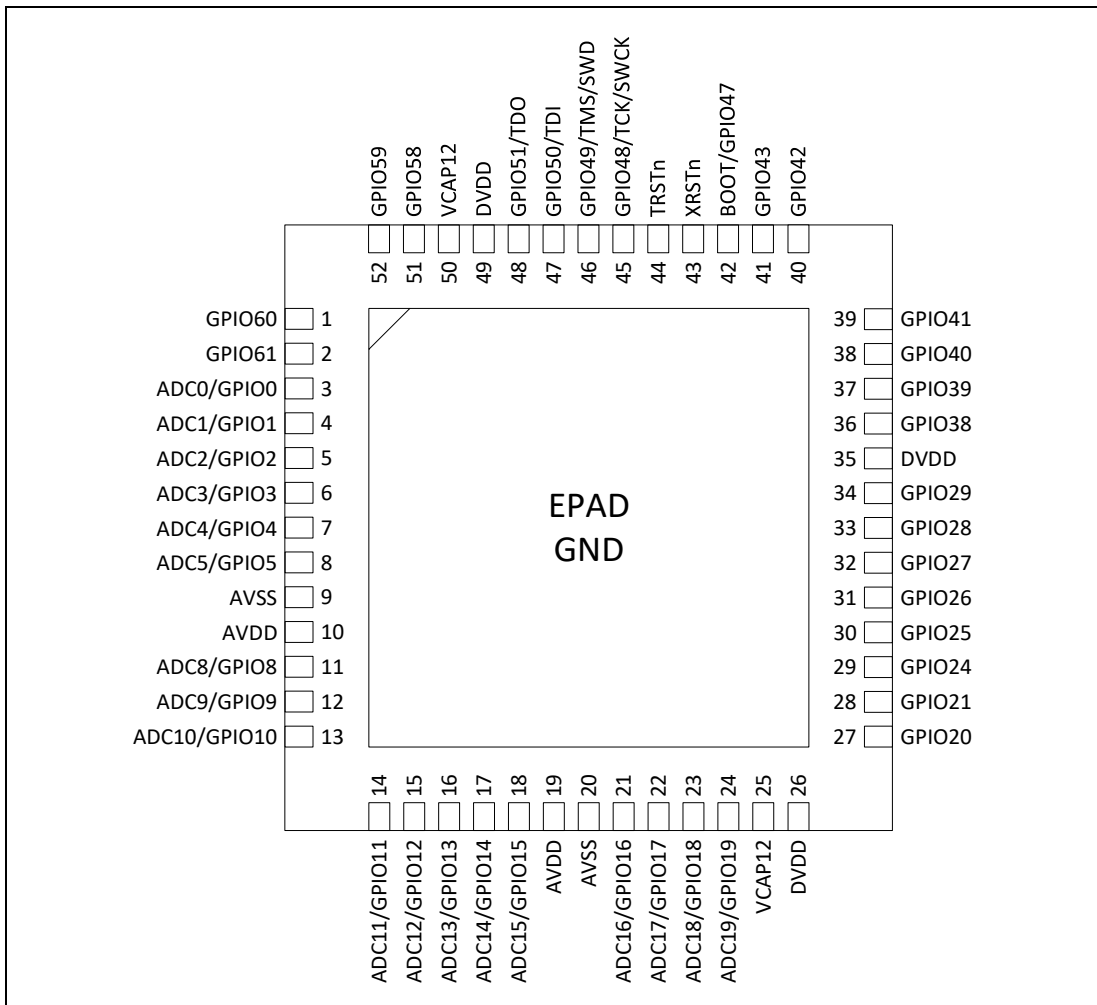
Figure 7. SPC1198 QFN52 pinout
