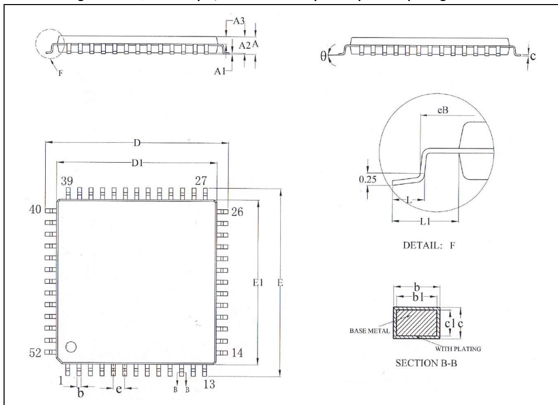
Figure 22. LQFP52 - 52 pin, 14 x 14 mm low-profile quad flat package outline
