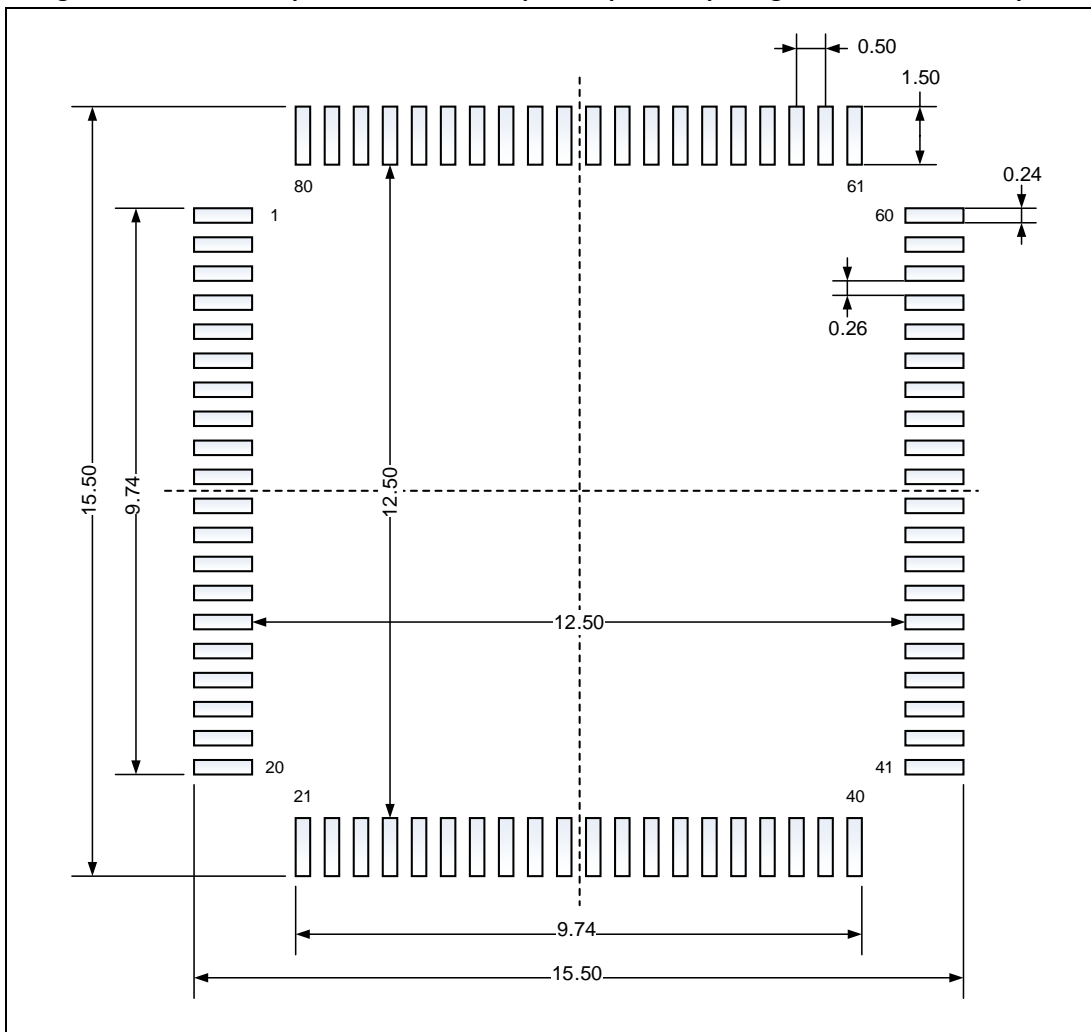
Figure 19. LQFP80 - 80 pin, 12 x 12 mm low-profile quad flat package recommended footprint
