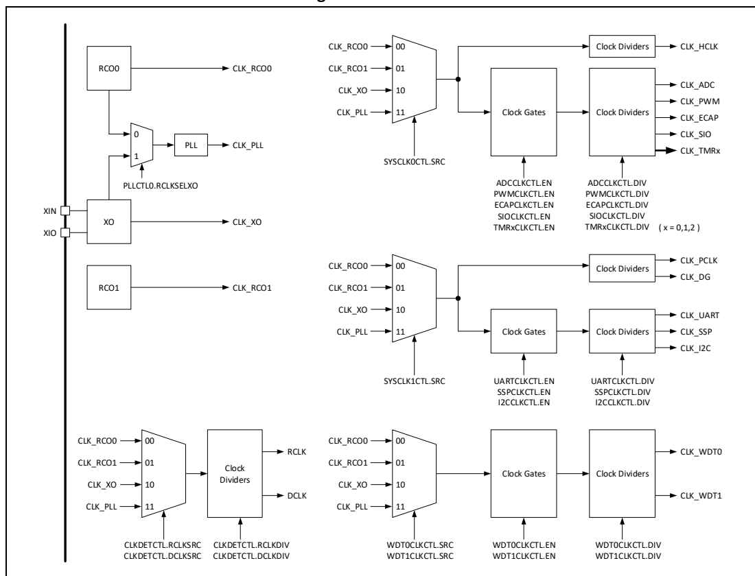
Figure 2. Clock tree
