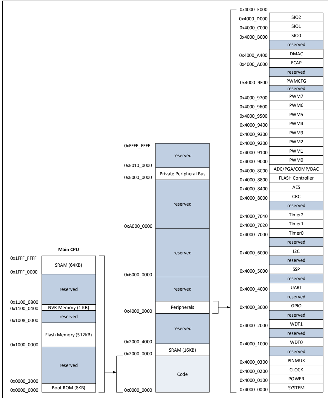
Figure 8. SPC1198 memory map with no Cache
