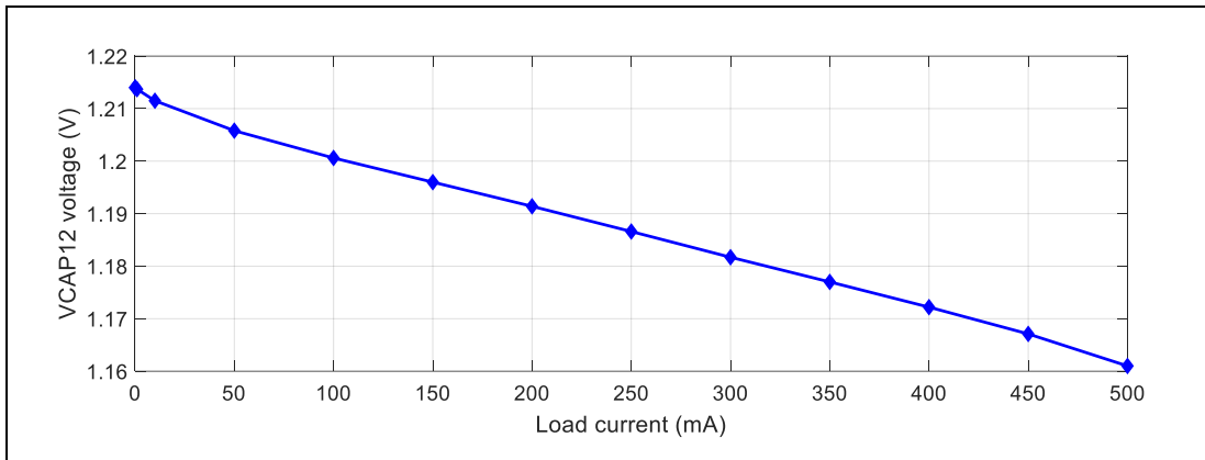
Figure 11. Internal 1.2V regulator load regulation ( T_A = 25 \text{ °C} )
