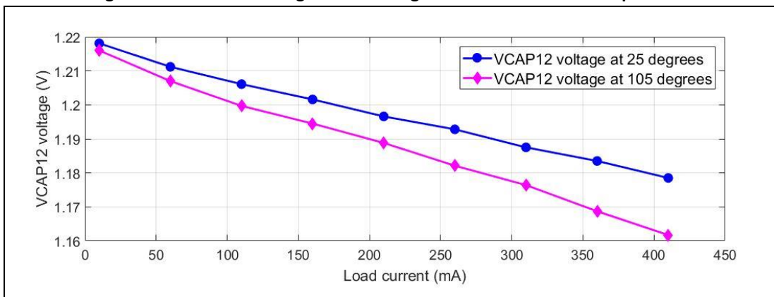
Figure 12. Internal 1.2V regulator load regulation with different temperature
