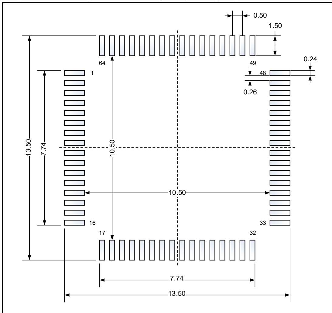
Figure 21. LQFP64 - 64 pin, 10 x 10 mm low-profile quad flat package recommended footprint
