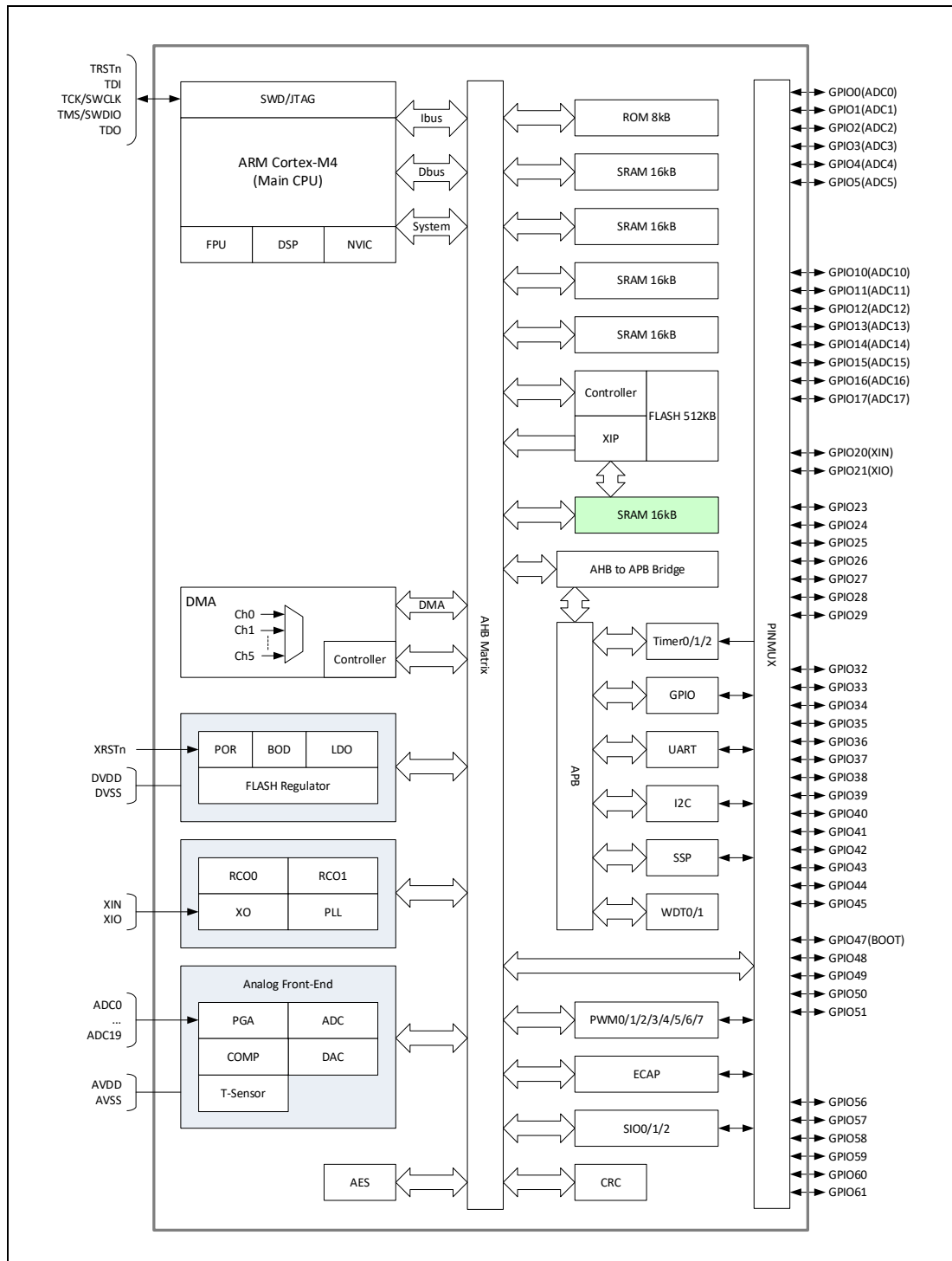
Figure 1. Block diagram of SPC1198
