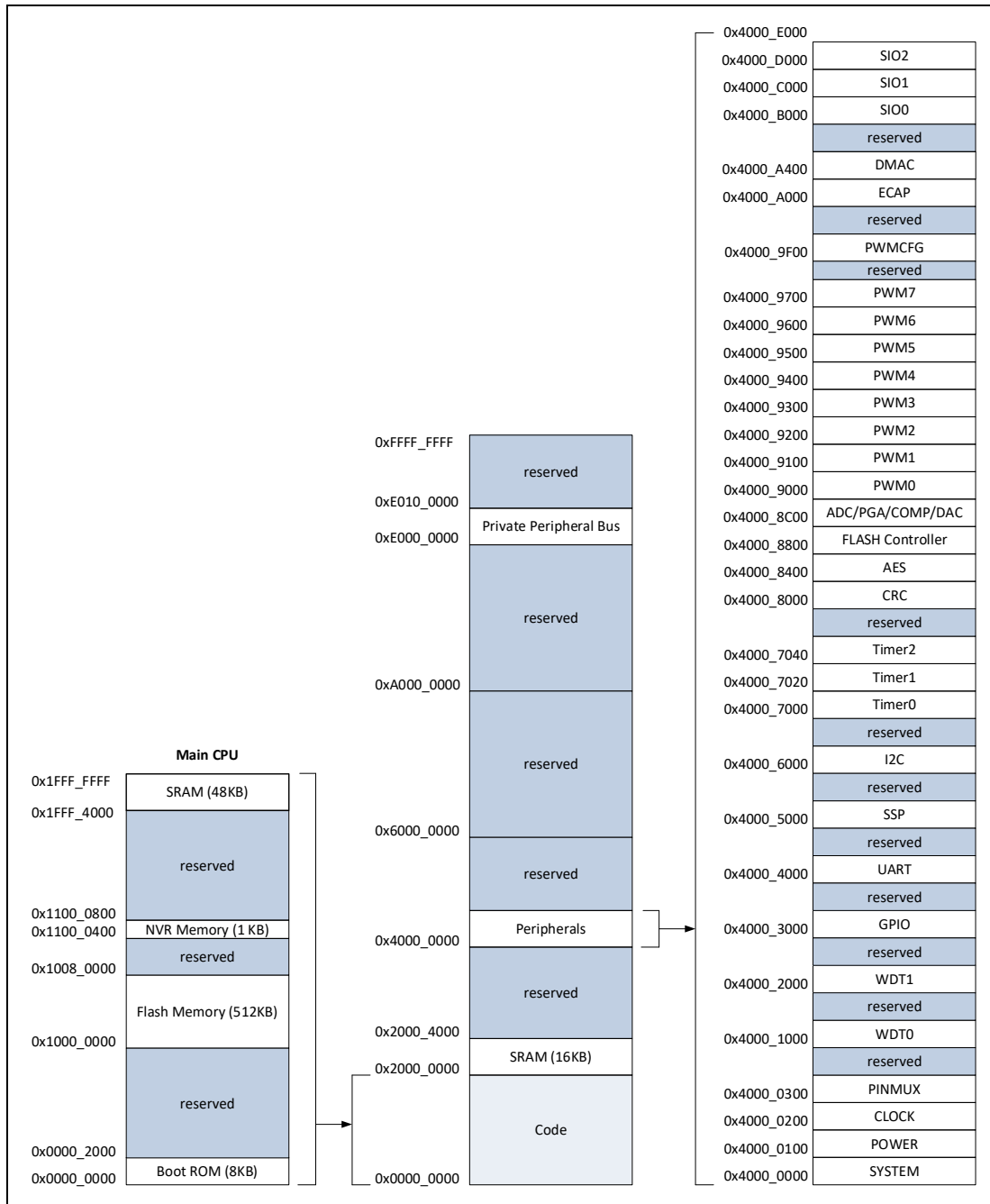
Figure 9. SPC1198 memory map with Cache
