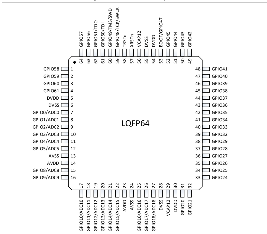
Figure 4. SPC1198 LQFP64 pinout
