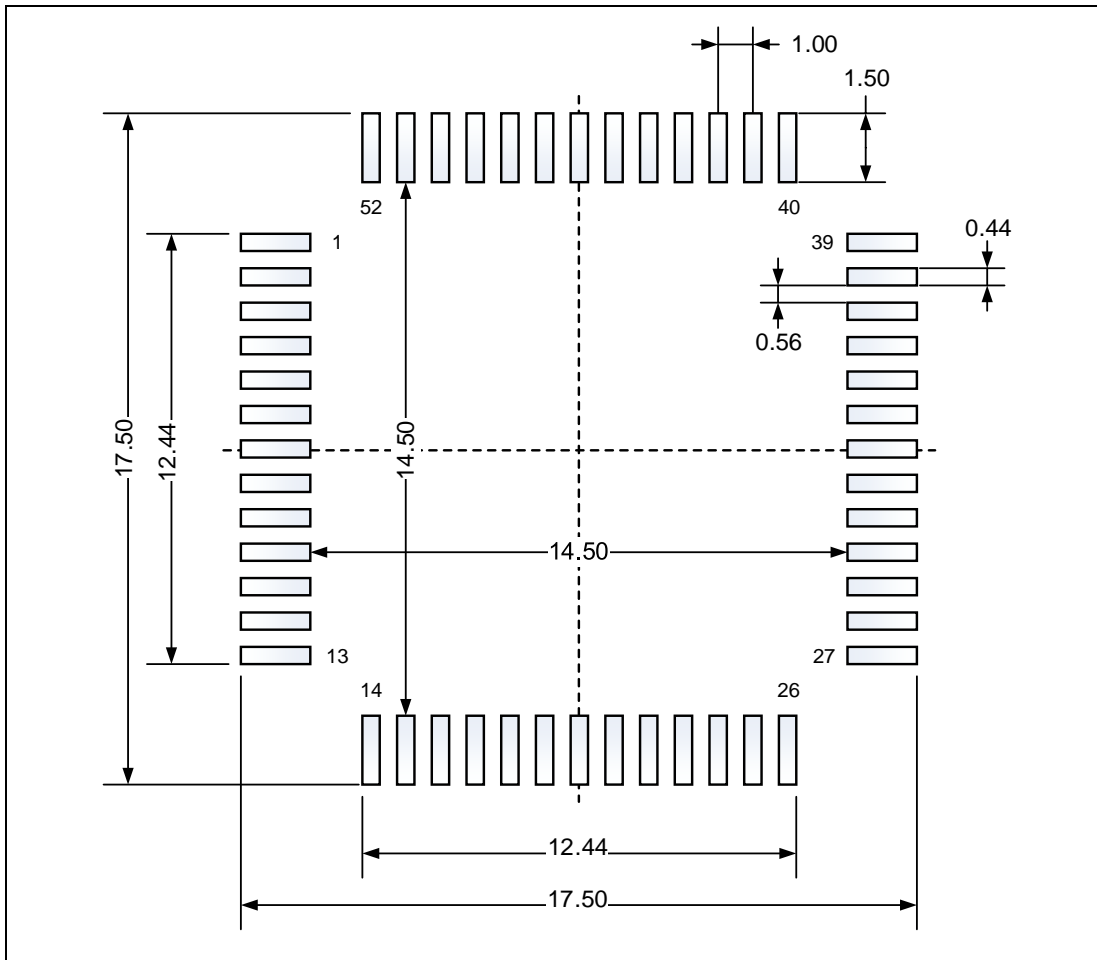
Figure 23. LQFP52 - 52 pin, 14 x 14 mm low-profile quad flat package recommended footprint
