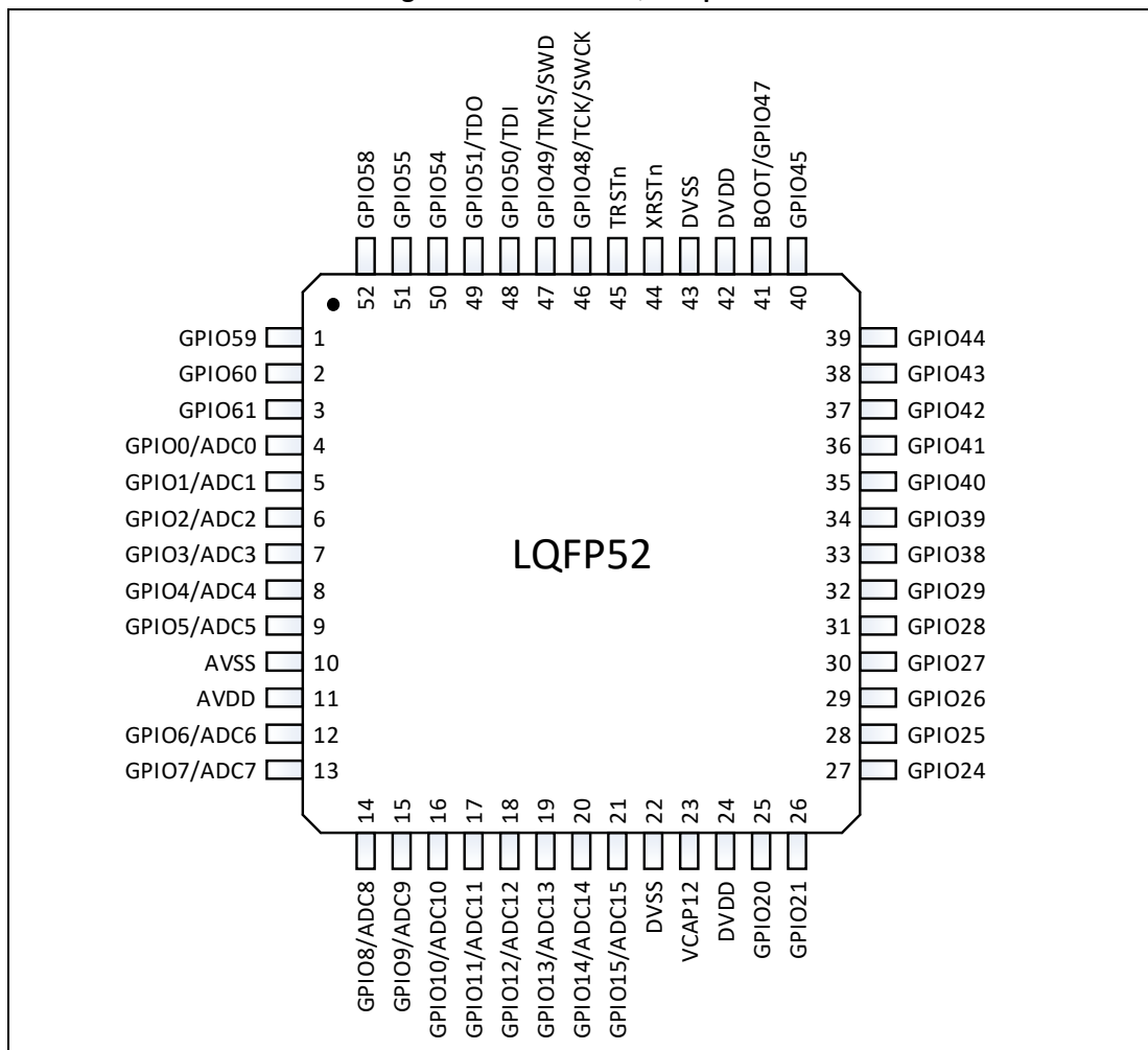
Figure 5. SPC1198 LQFP52 pinout
