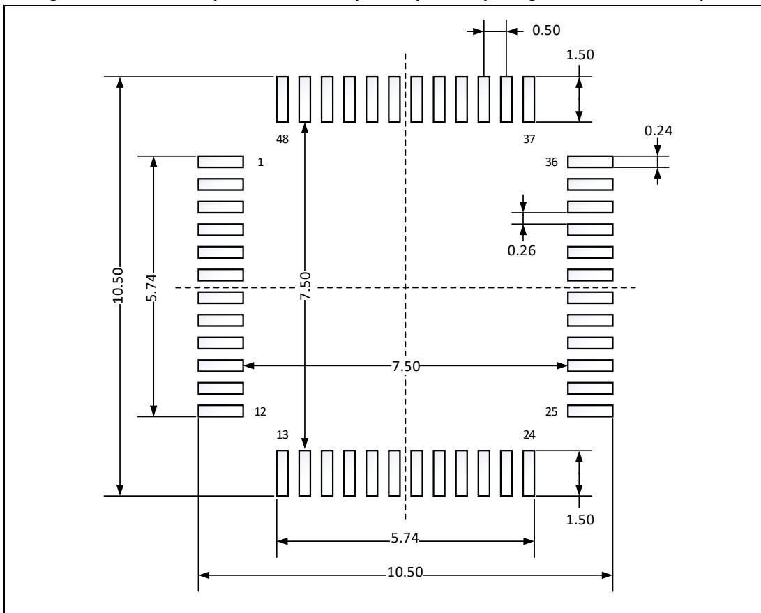
Figure 25. LQFP48 - 48 pin, 7 x 7 mm low-profile quad flat package recommended footprint
