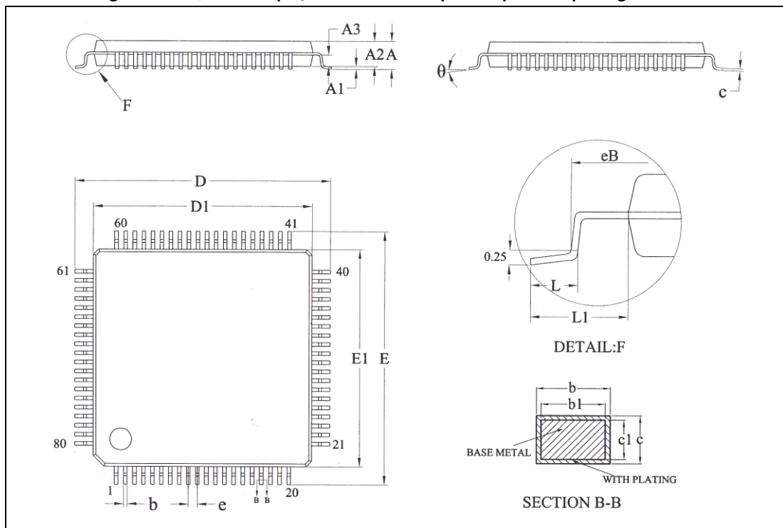
Figure 20. LQFP64 - 64 pin, 10 x 10 mm low-profile quad flat package outline
