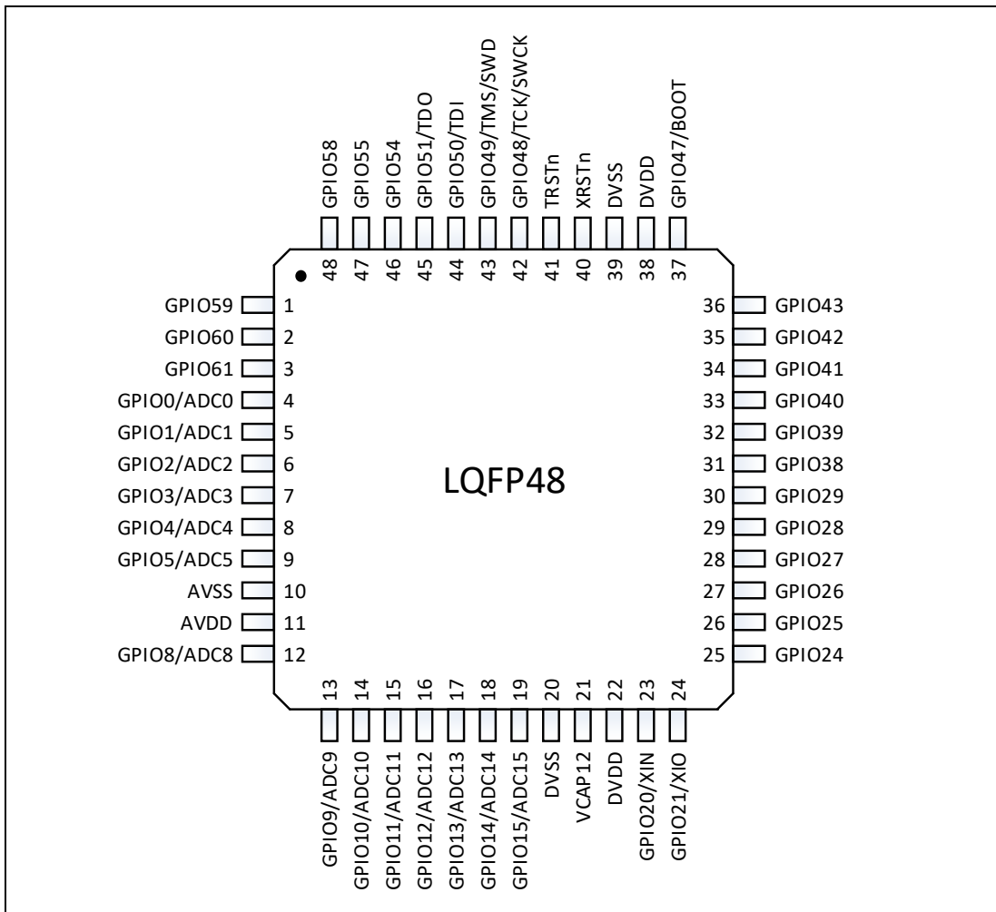
Figure 6. SPC1198 LQFP48 pinout
