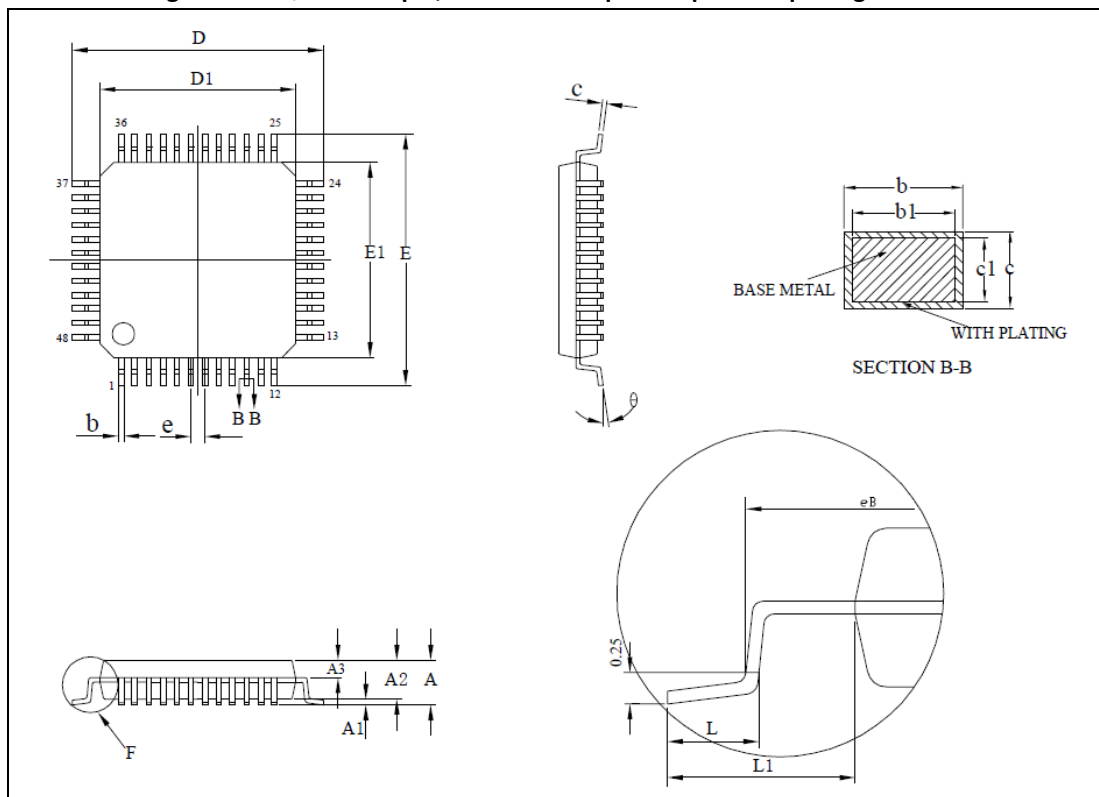
Figure 24. LQFP48 - 48 pin, 7 x 7 mm low-profile quad flat package outline
