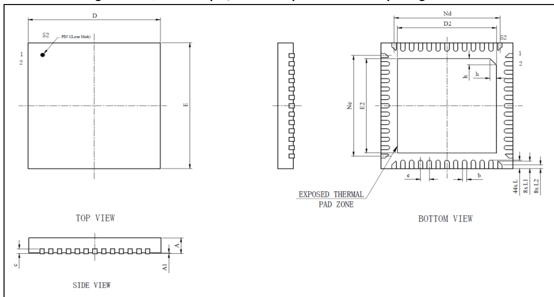
Figure 26. QFN52 - 52 pin, 6 x 6 mm quad flat no-lead package outline
